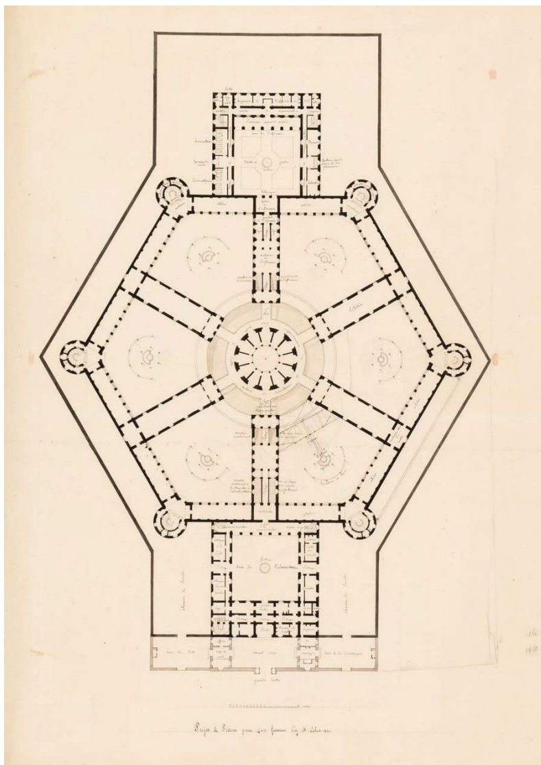
Fig.7 Îchisoarea Petit Roquette, plan, 1826 arh. Louis-Hippolyte Lebas, Collection Centre Canadien d'Architecture/ Canadian Centre for Architecture, Montréal https://www.cca.qc.ca/en/search/details/collection/object/2036 consultat în data de 22 august 2024
